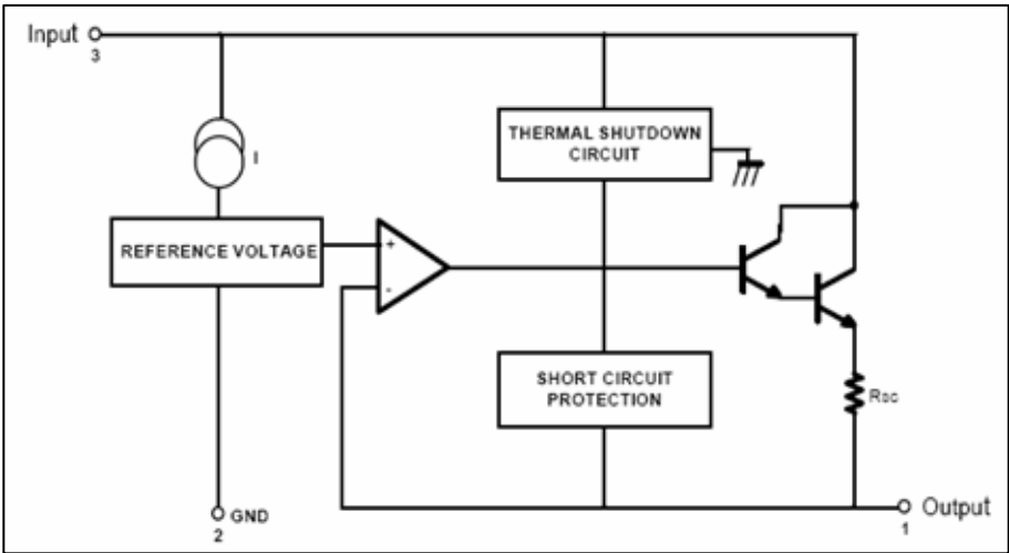
Block Diagram
