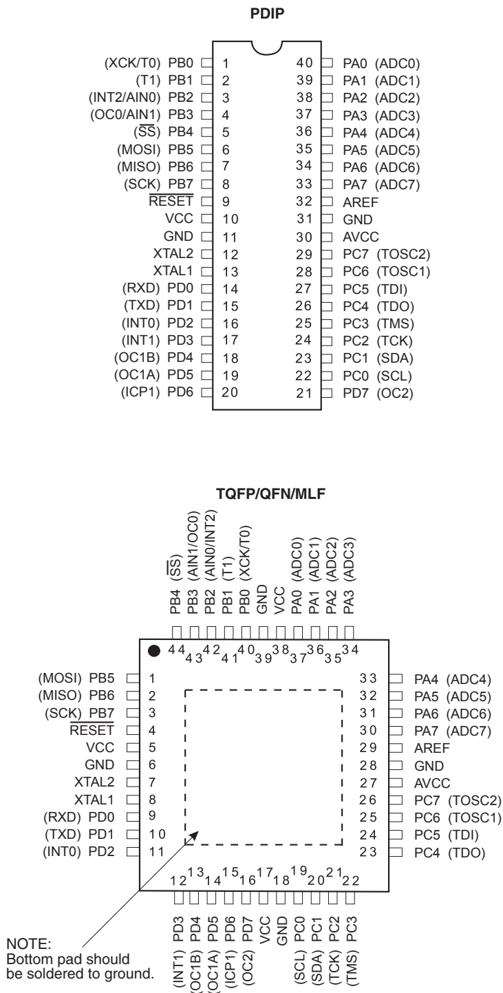
Figure 1-1. Pinout ATmega16A
