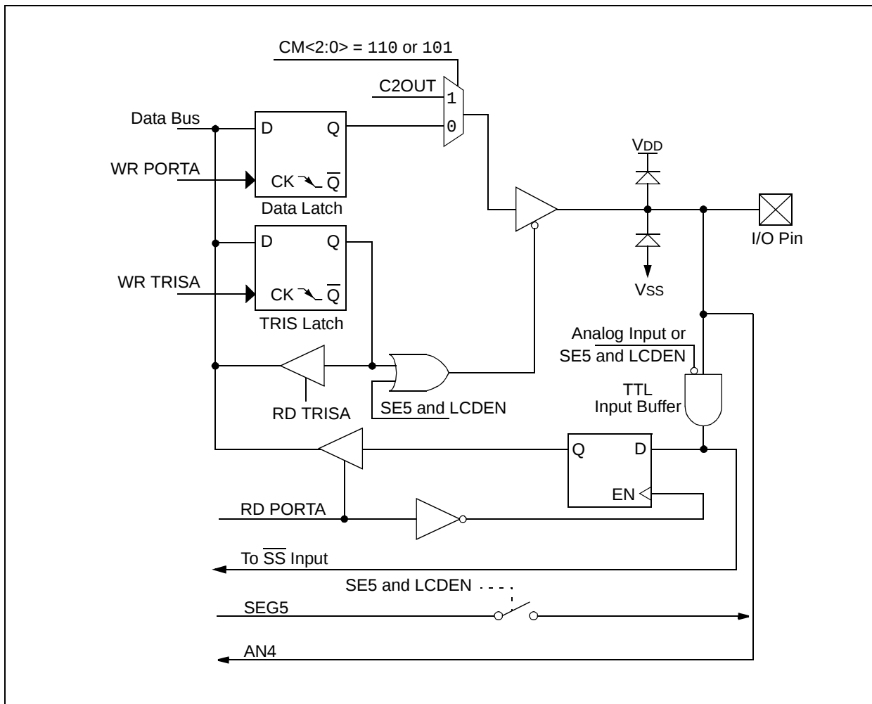
FIGURE 4-6: BLOCK DIAGRAM OF RA5/AN4/C2OUT/SS/SEG5
