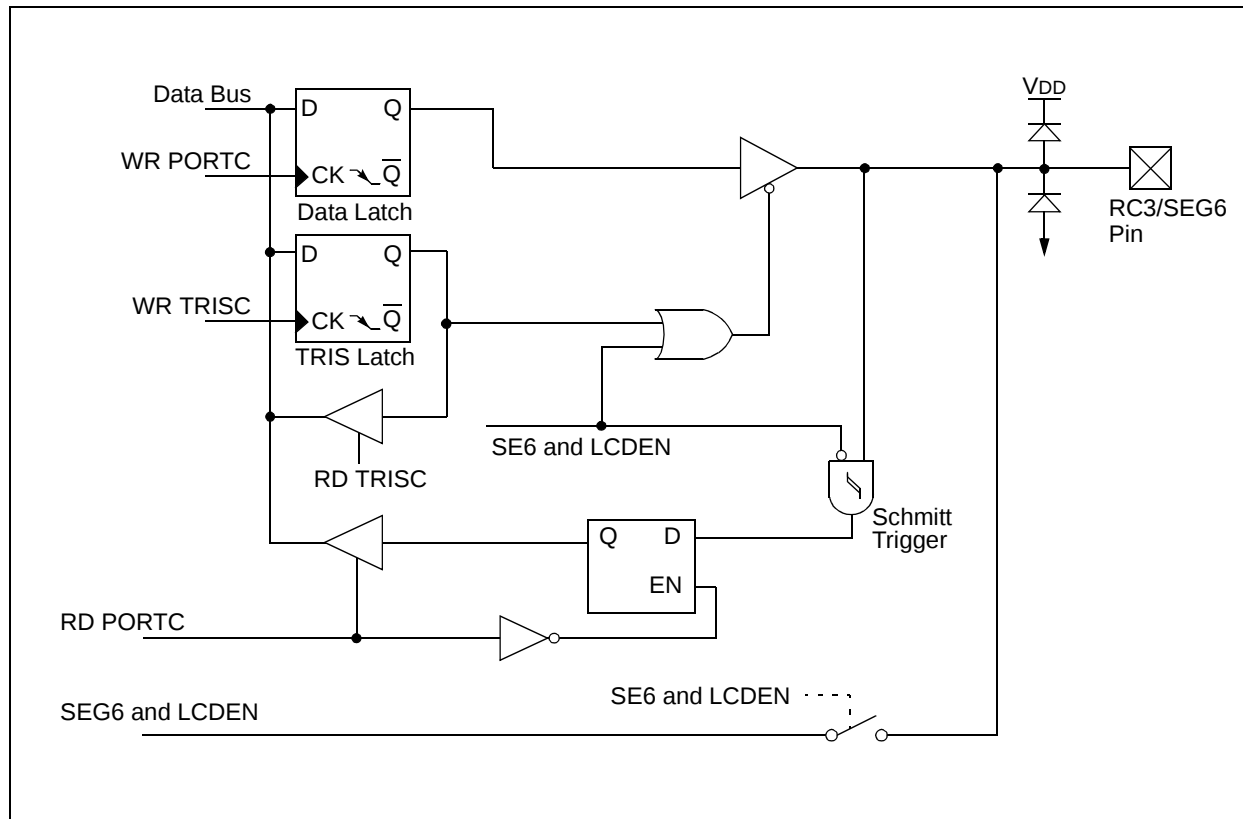
FIGURE 4-17: BLOCK DIAGRAM OF RC3/SEG6
