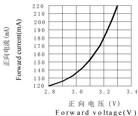
电流与电压 Current and voltage
